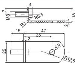
UXP-100F Terminals
