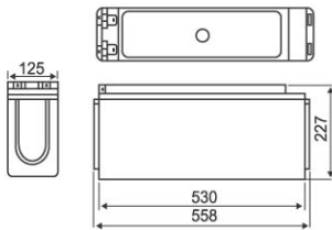
UXP-100F Terminals
