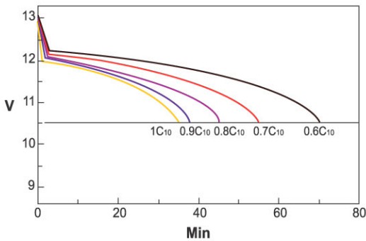
Fig. 0.6C 10 ~1C 10 A Discharge curves
