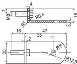
UXP-100F Terminals
