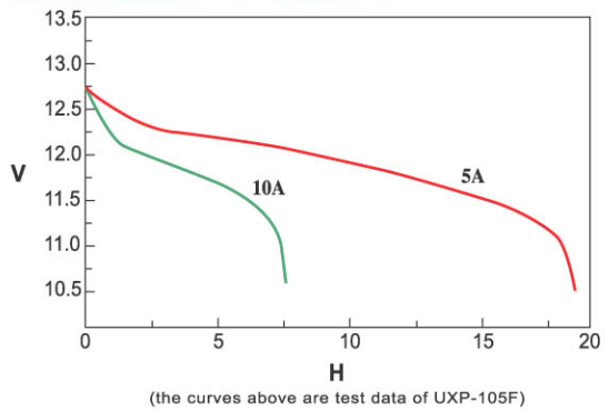
Fig. Discharge curves at 5A \ 10A(-15°C/10.50v)
