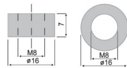
UXP-100M, UXP-200M Terminals
